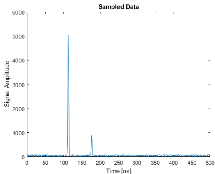
Figure 4: Emitted EDM pulses on RTC360.
