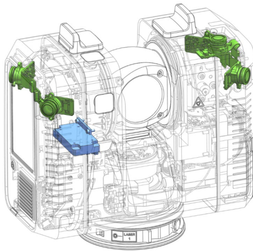
Figure 6: Hardware components of the Visual Inertial System.
