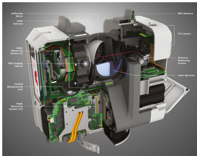
Figure 2: A look inside the RTC360
