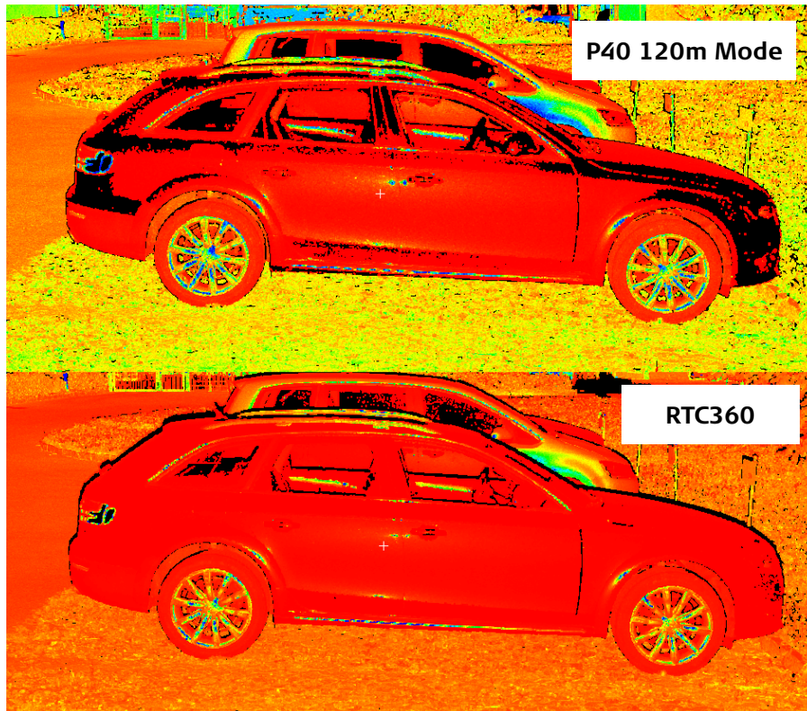
Figure 5: Comparison of the same scan of a black car performed with ScanStation P40 and RTC360..
